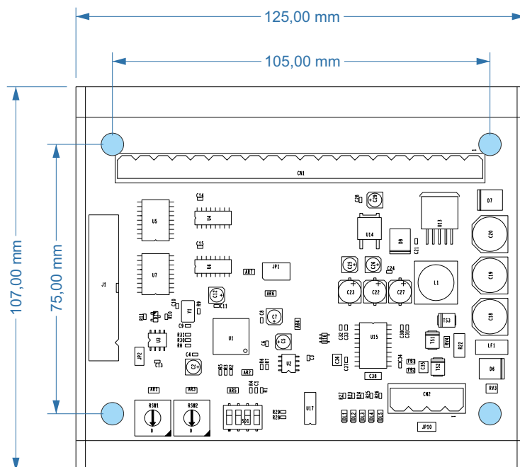
Figure 4) Module dimensions
