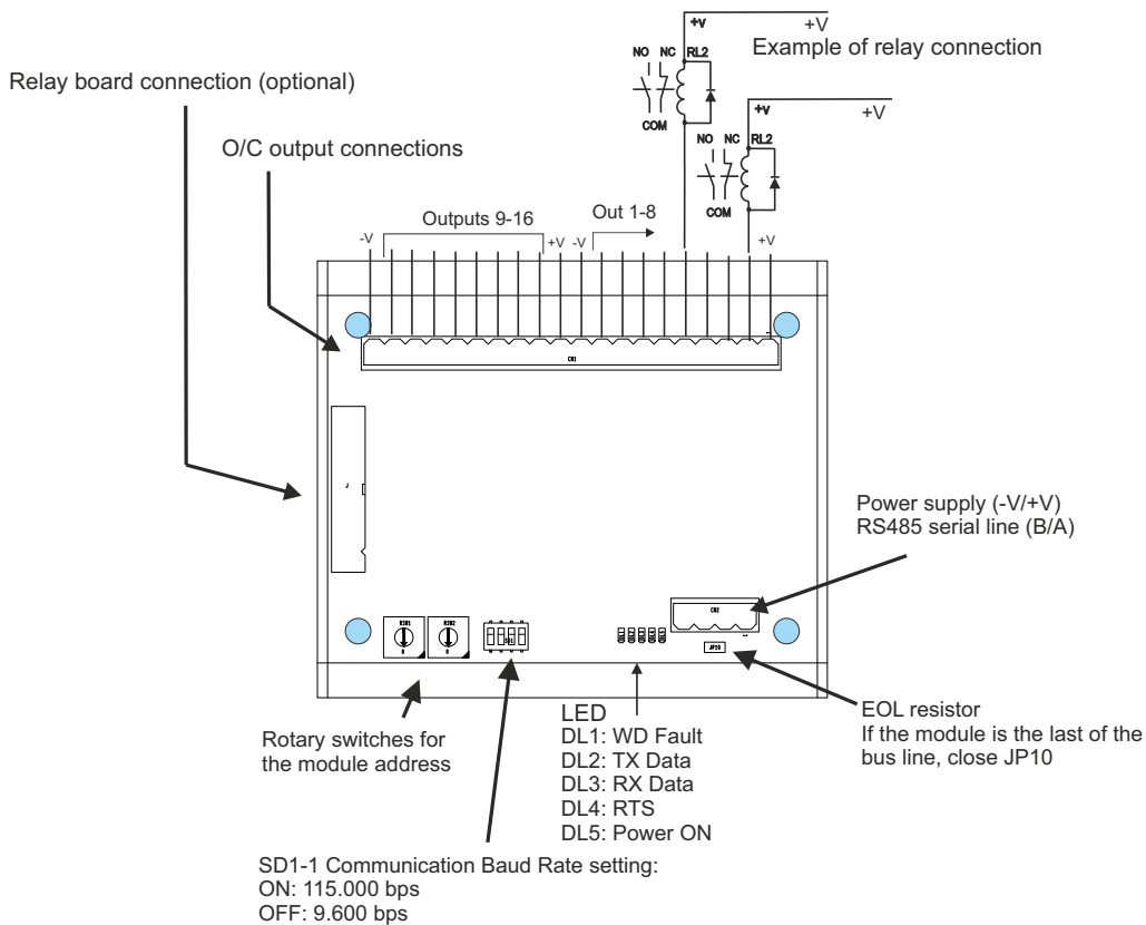
Figure 1) Layout STG/IN8S
