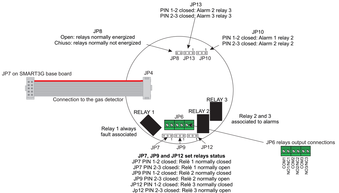
Figure 3) Inside view of SMART3G display
