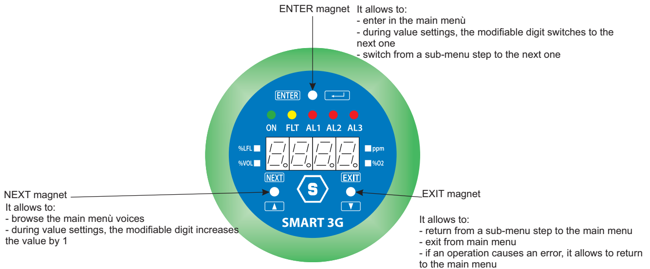
Figure 4) Description of ENTER, NEXT and EXIT magnets
