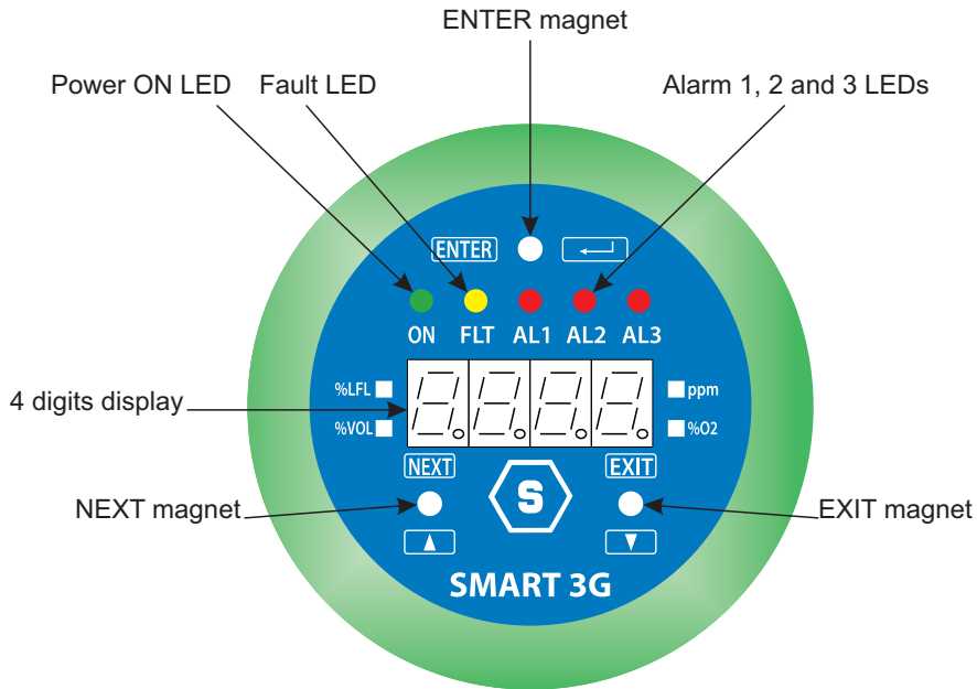
Figure 2) Front view of SMART3G display
