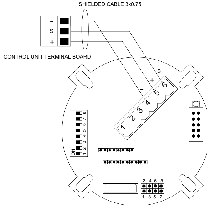
Figure 2) Connection scheme for the 4-20 mA output
