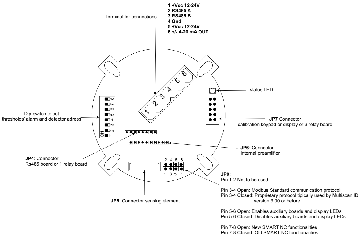
Figure 1) Detector circuit layout
