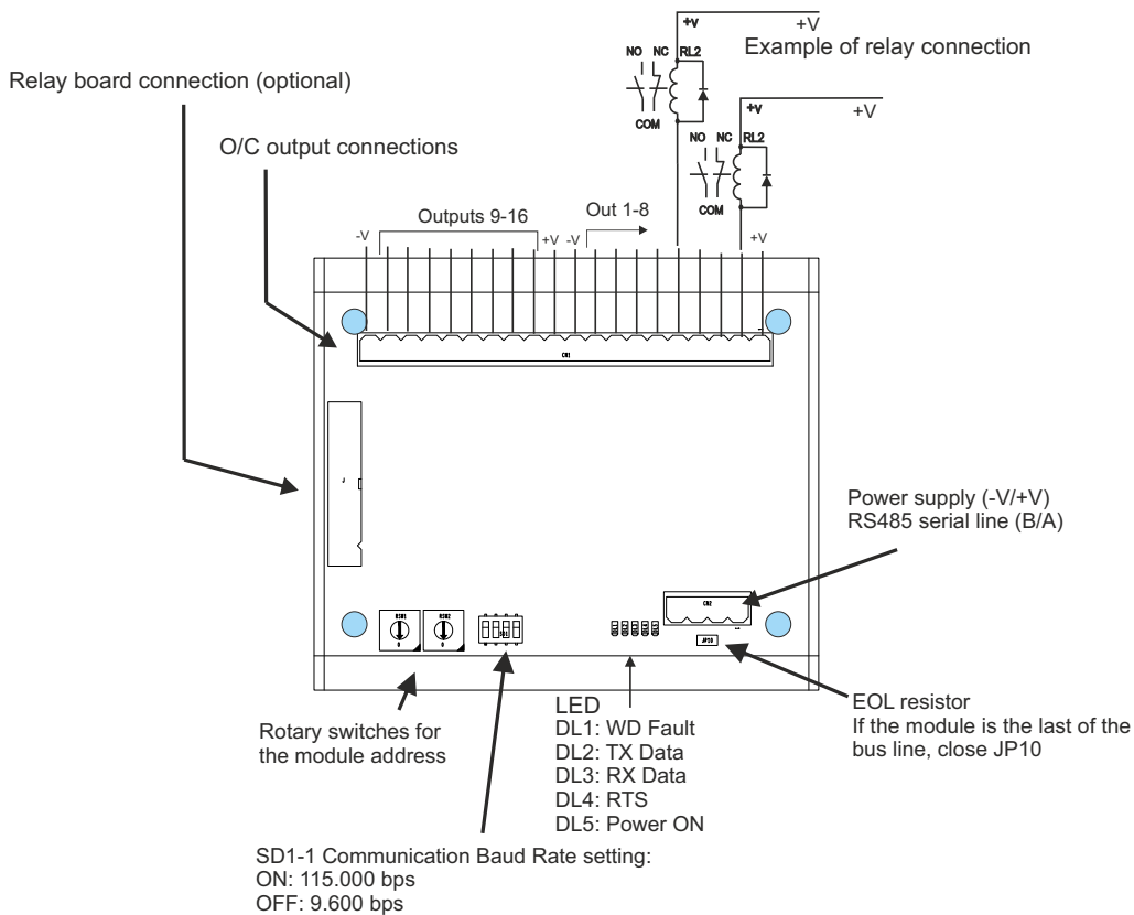
Figure 1) Layout STG/IN85
