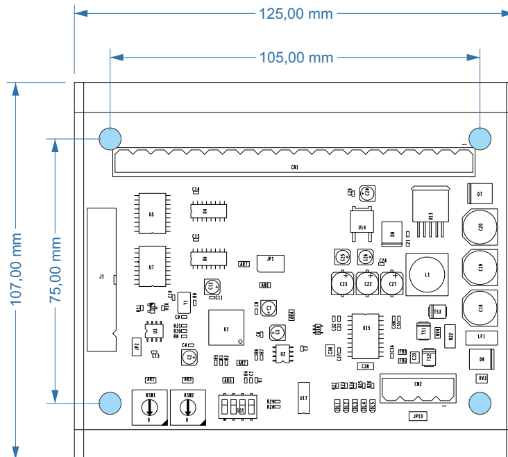
Figure 4) Module dimensions
