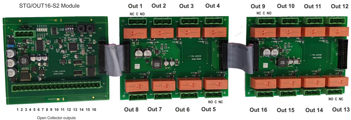
Figure 3) Relay board connection
