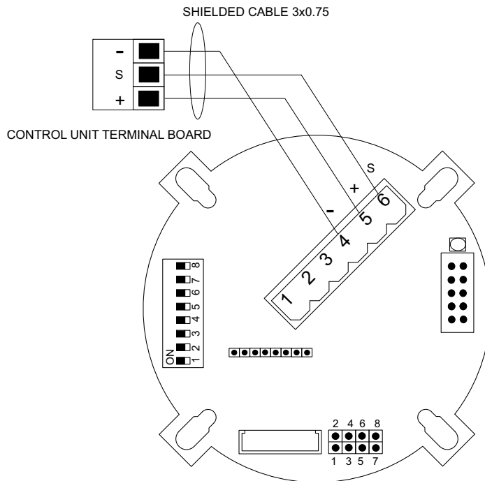
Figure 2) Connection scheme for the 4-20 mA output with shielded cable
