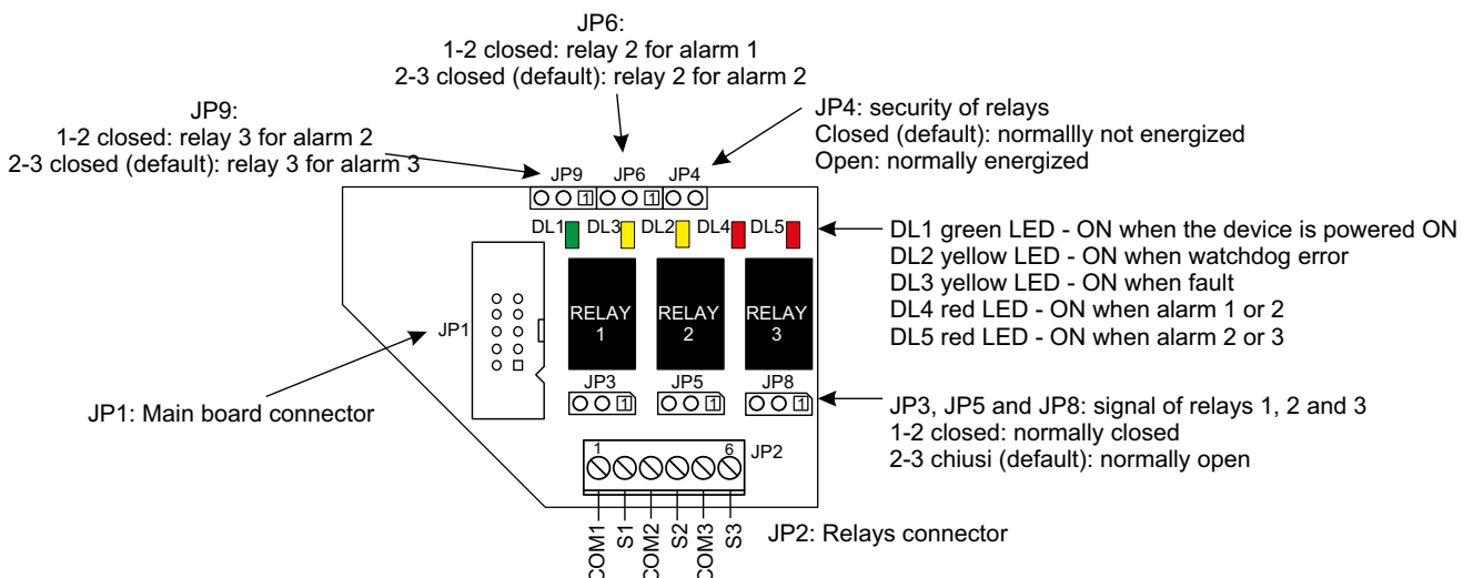
Figure 3) 3 relays board
