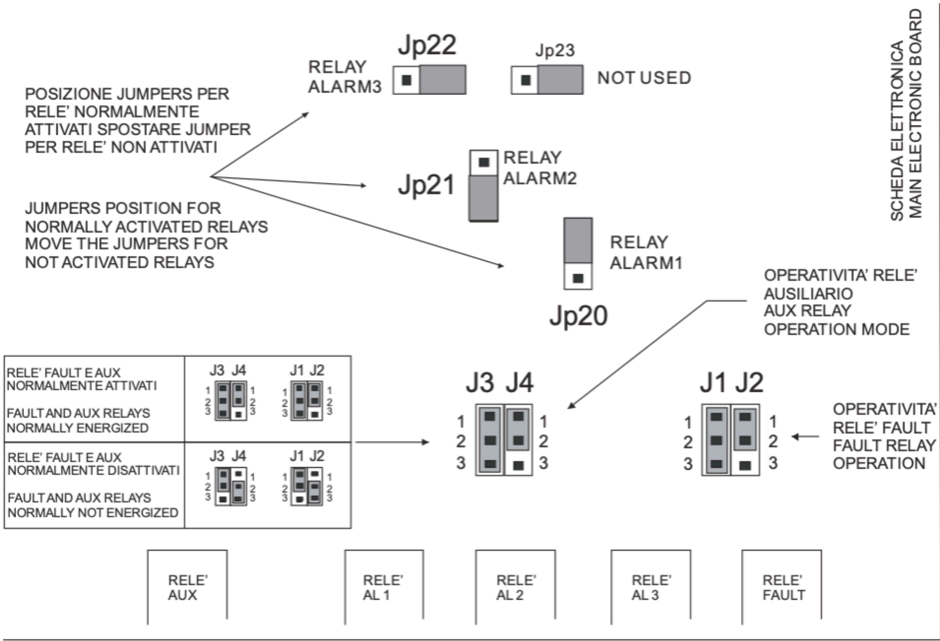
RELAYS OPERATION MODE
