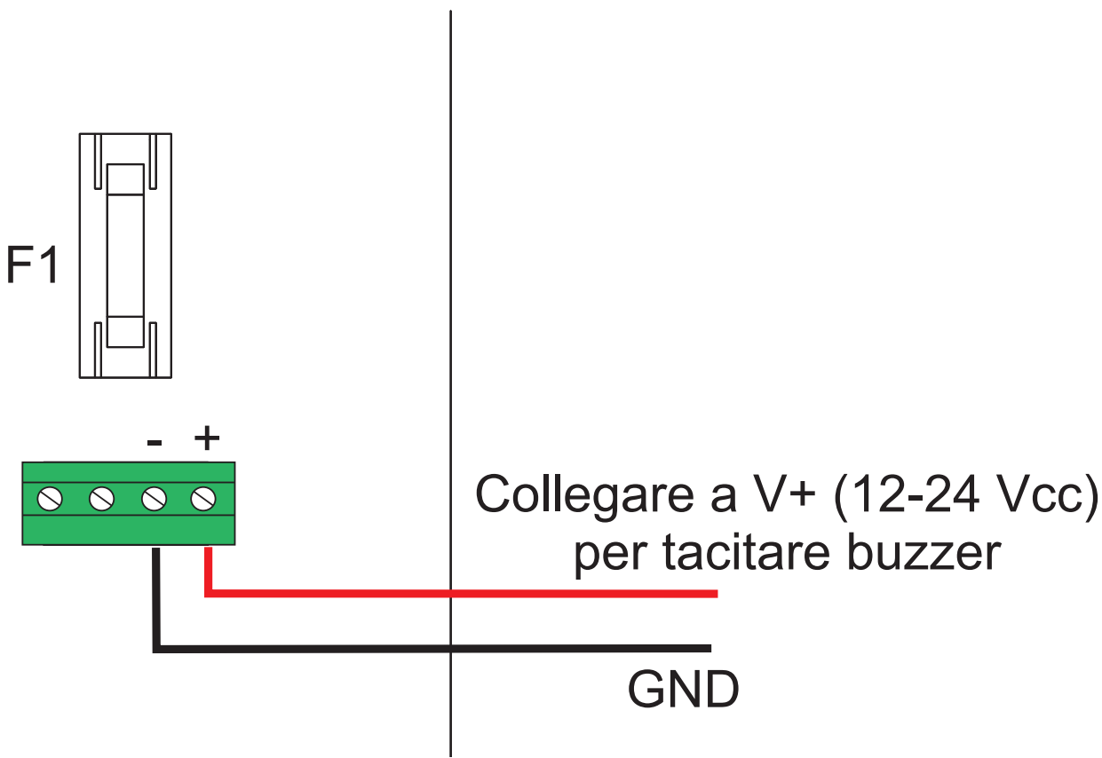
Figure 9 Digital input 1 connecction
