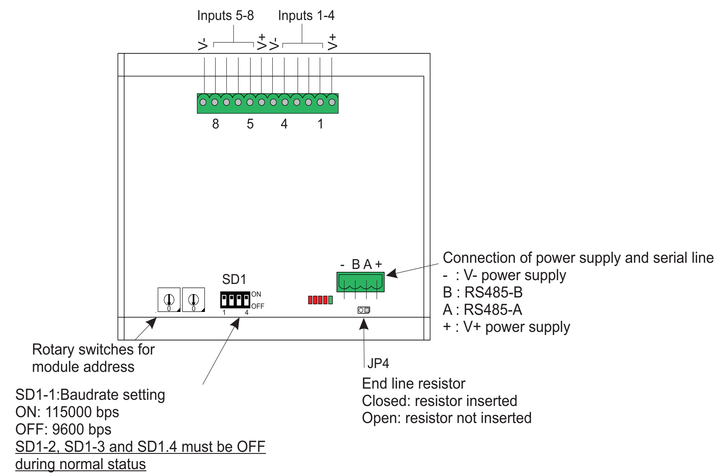
Figure 12 STG/IN8-S2 module
