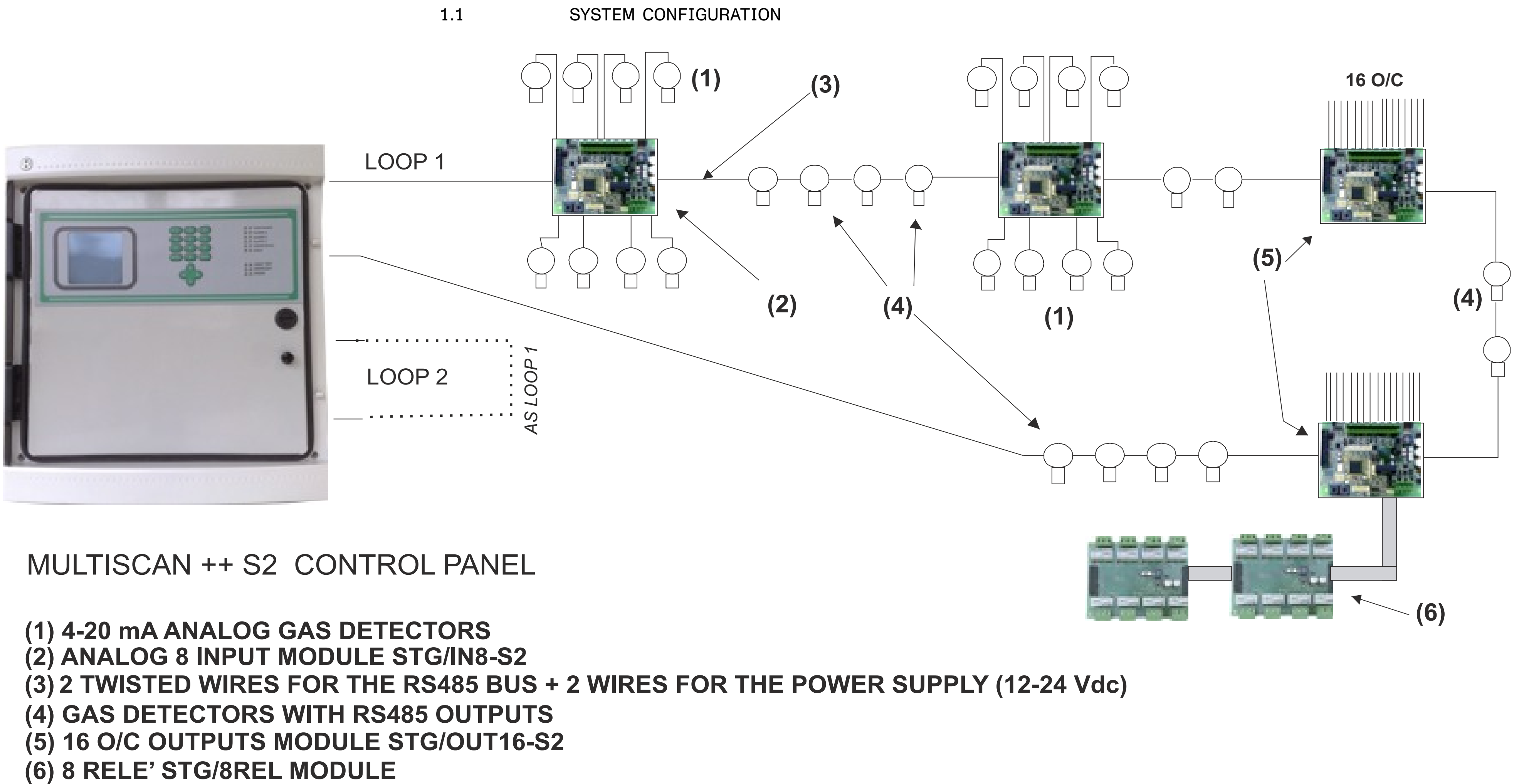
Figure 1 System block diagram Multiscan++S2
