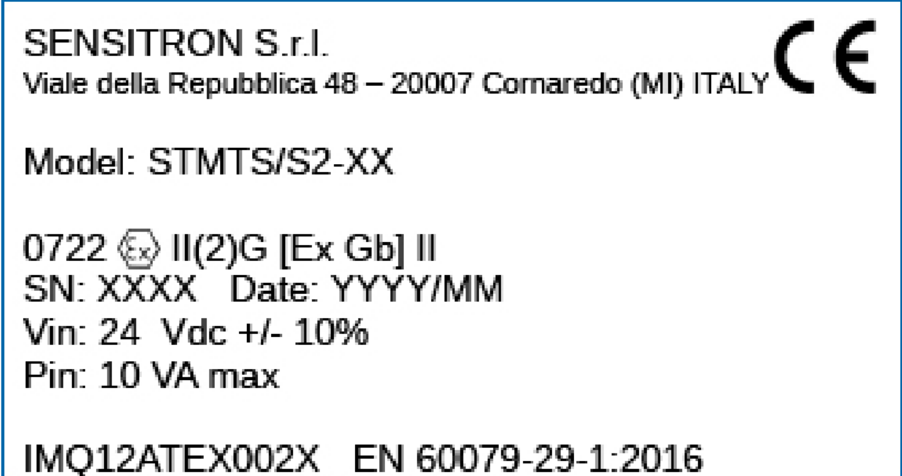
Figure 2 Example of ATEX and IECEx marking, rack version
