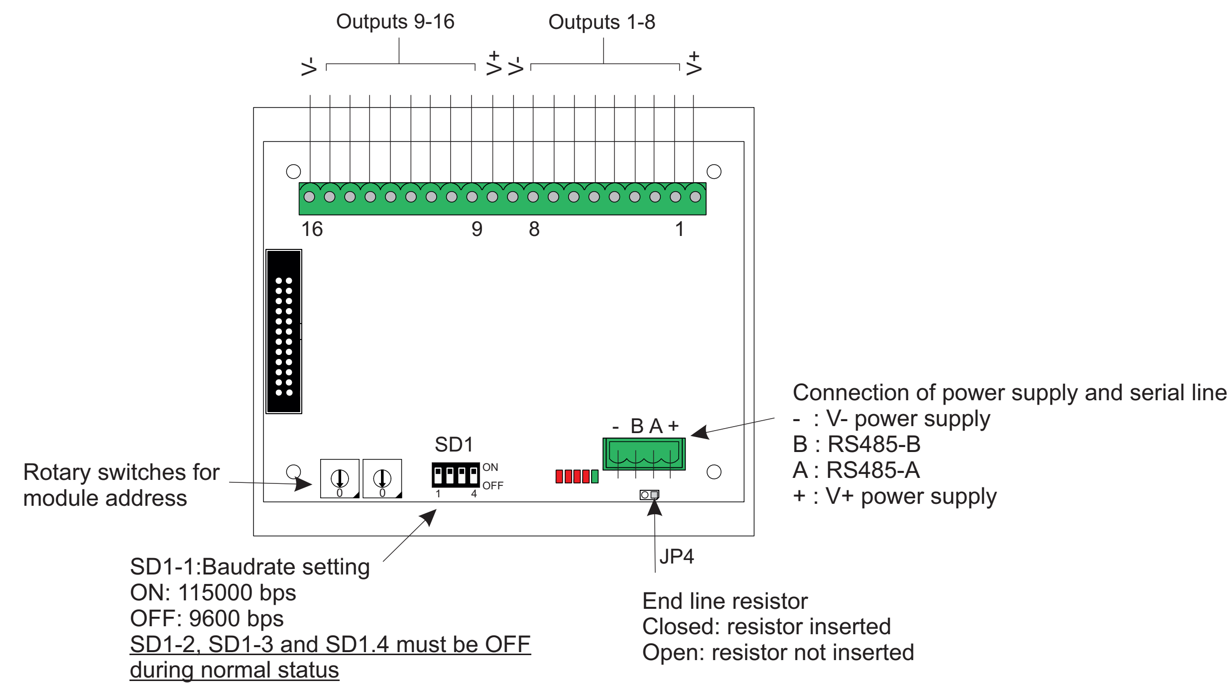
Figure 13 STG/OUT16-S2 module
