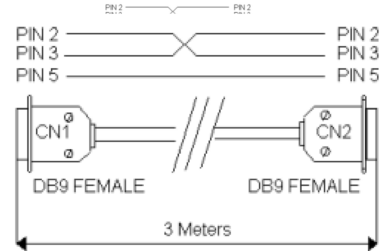
Figure 17 PC connection cable
