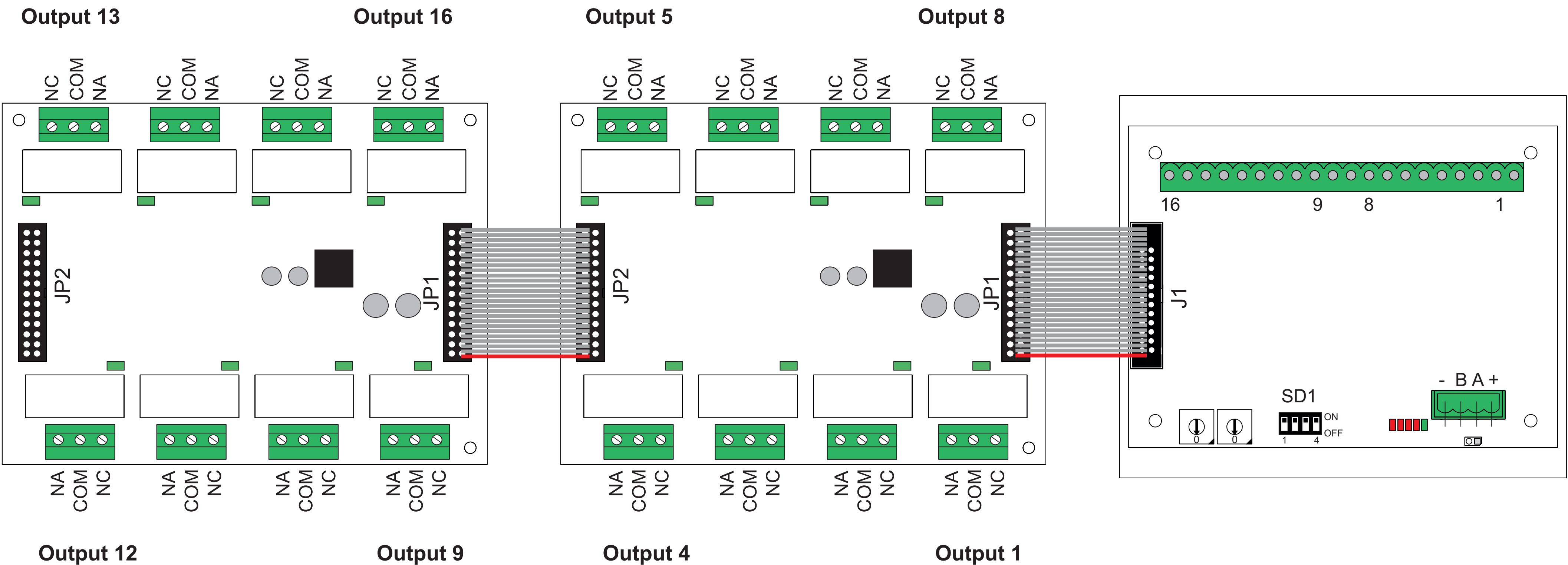
Figure 14 Relay board connection to the output module
