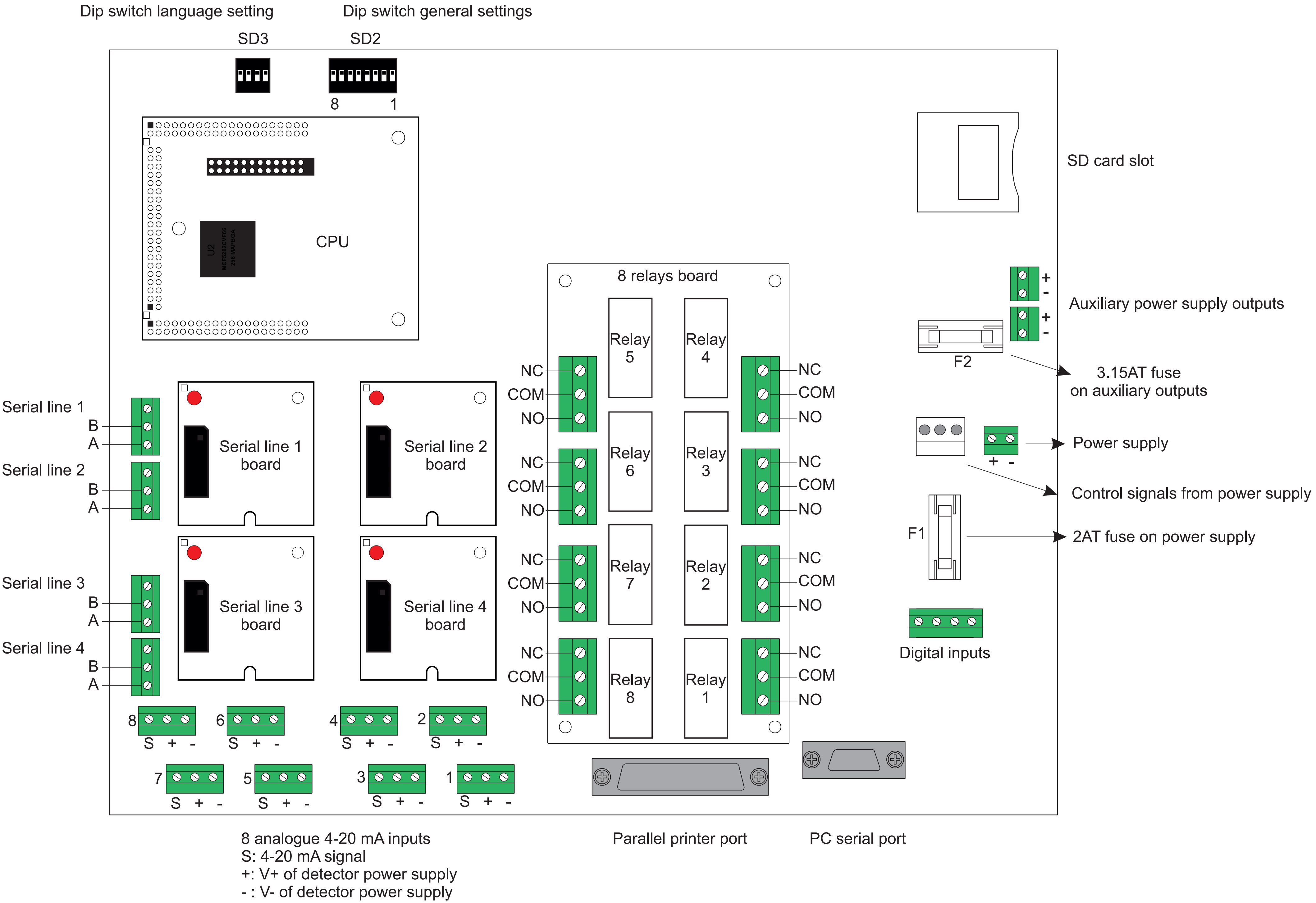
Figure 6 Layout main board
