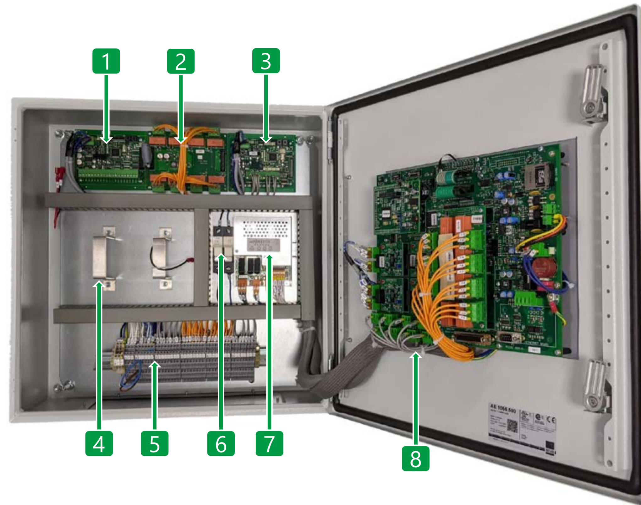
Figure 5 Overall view and part identification
