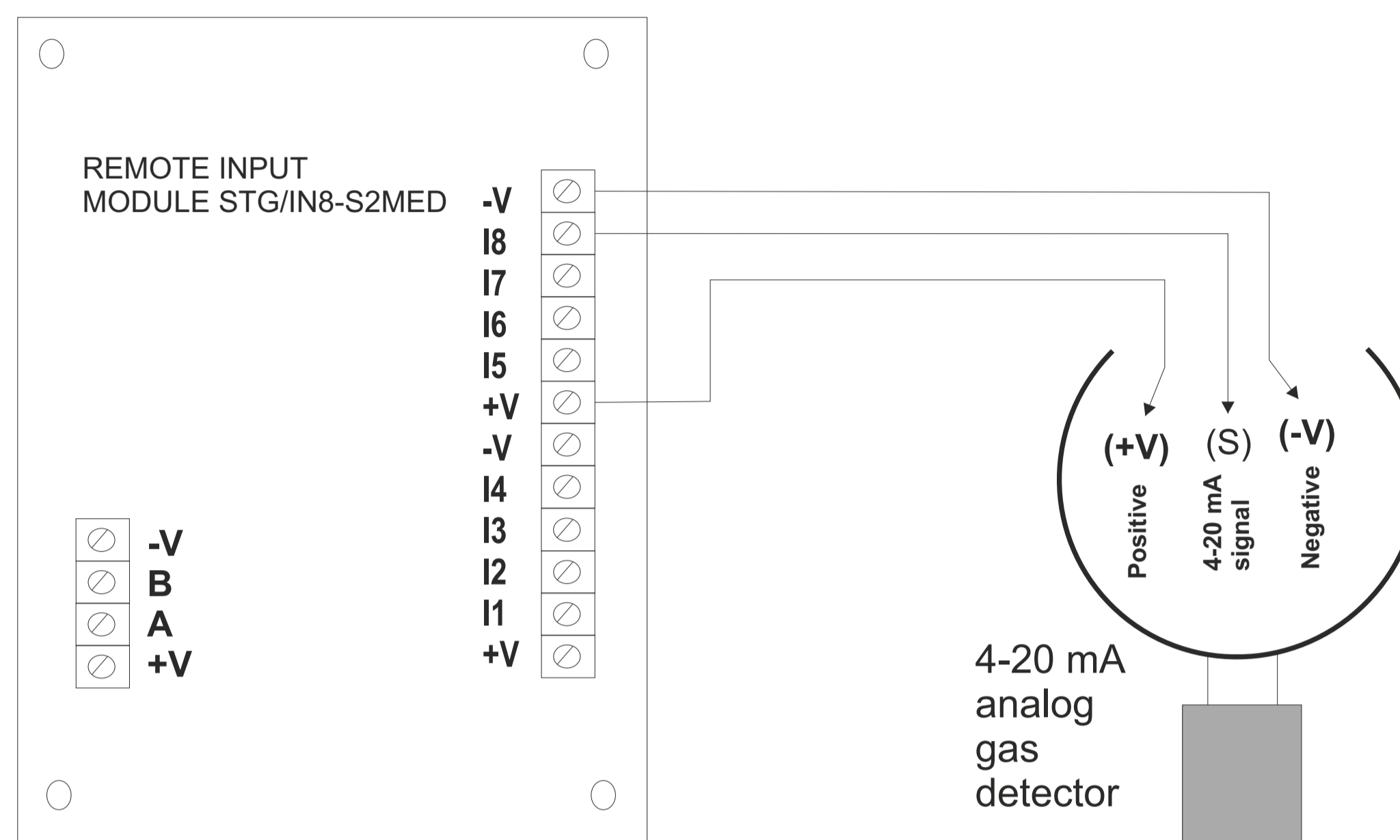
Figure 8 Connection of the 8 detectors of the STG/IN8-S2MED module
