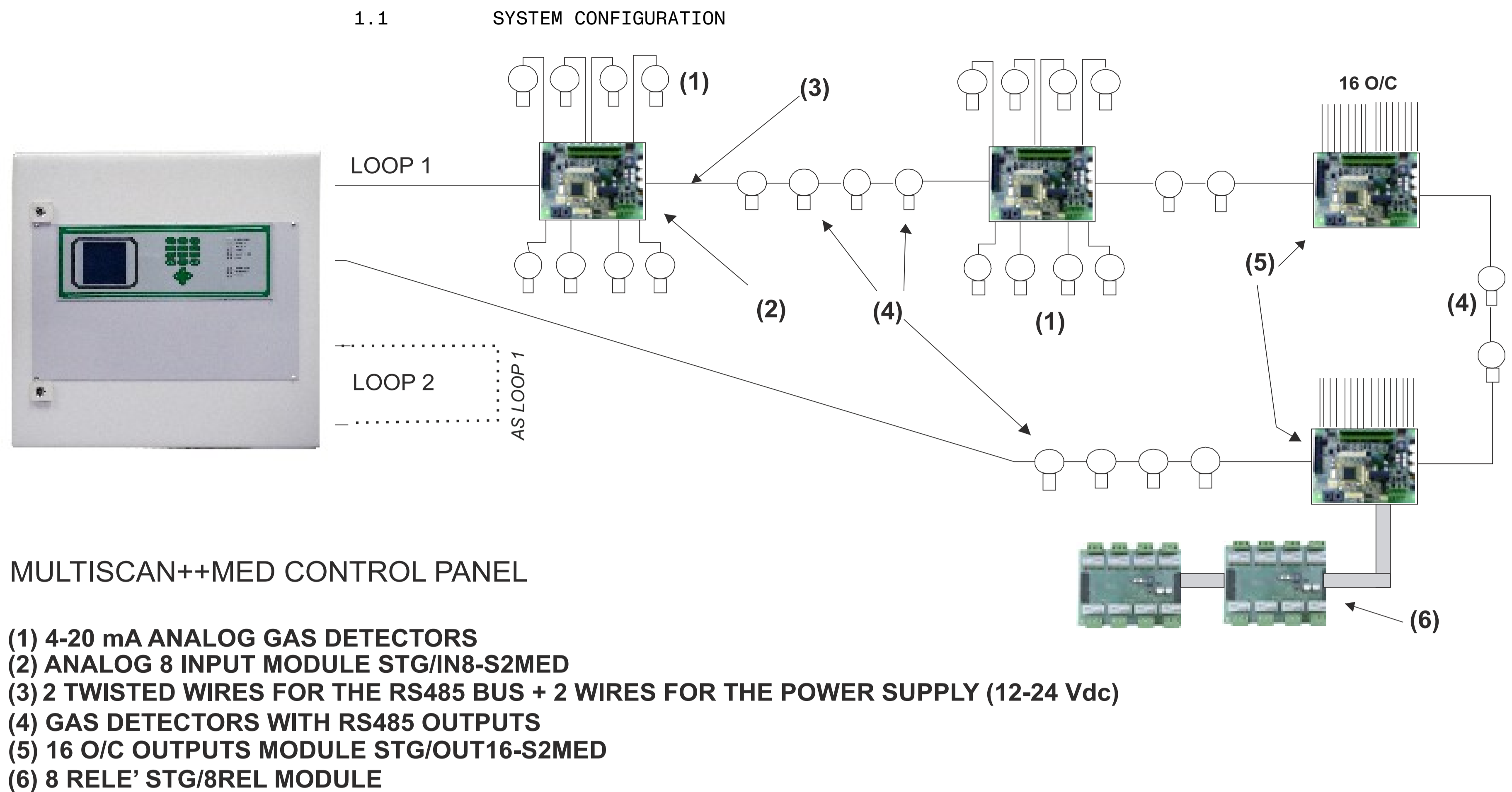
Figure 1 System block diagram MULTISCAN++MED
