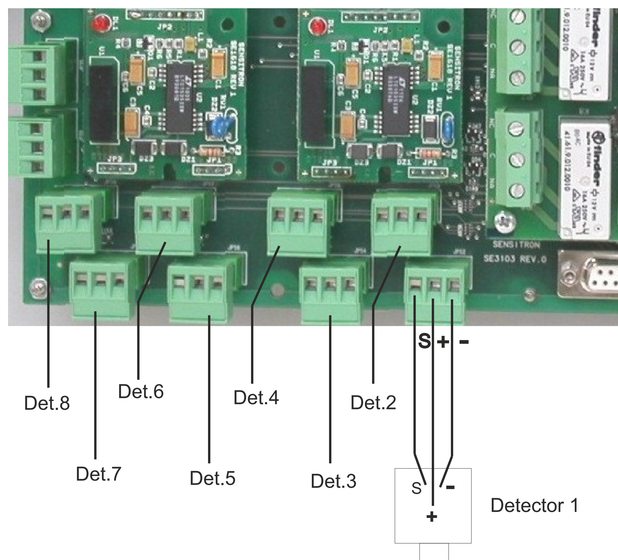
Figure 7 Connection of the 8 detectors to the control panel
