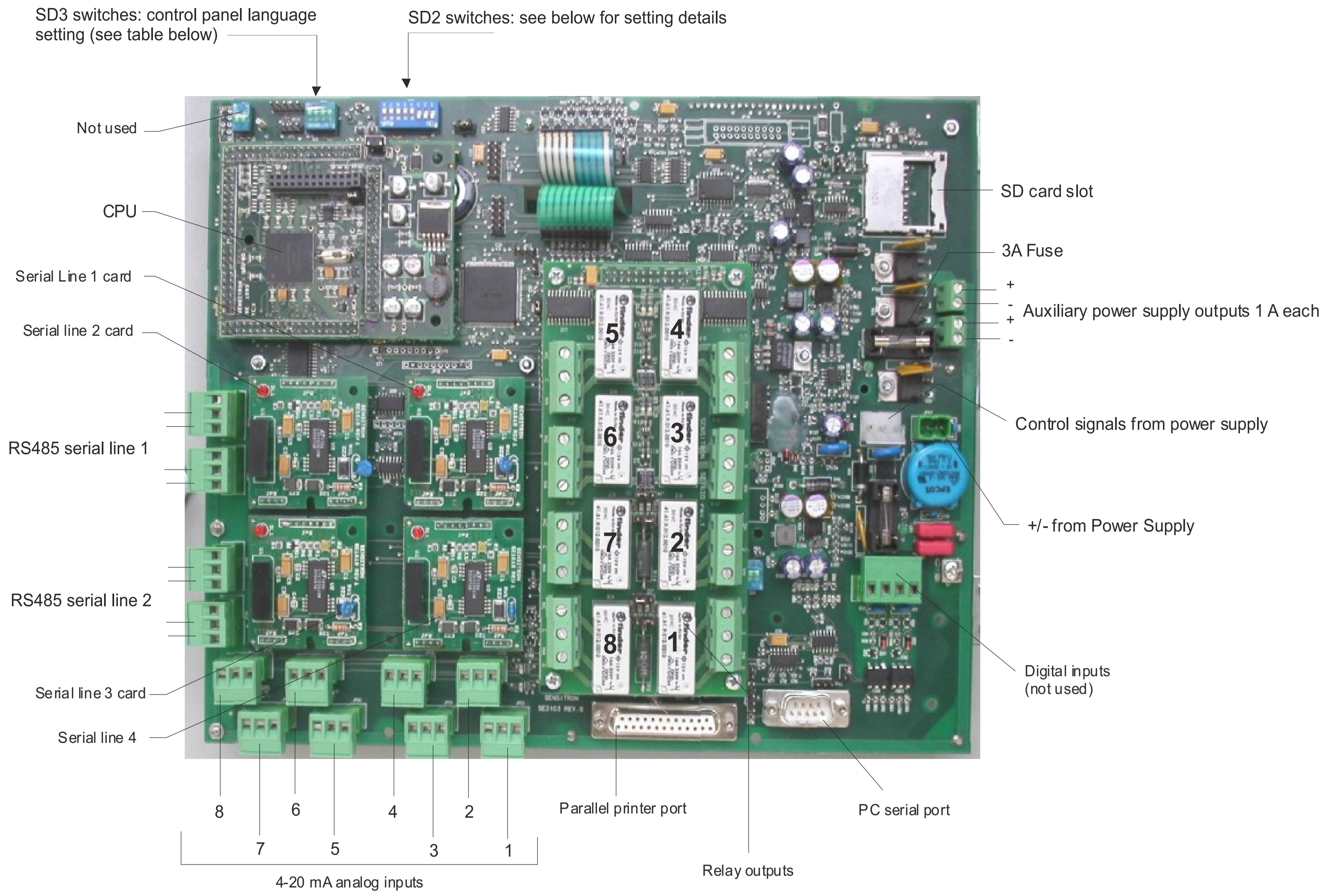
Figure 6 Layout main board
