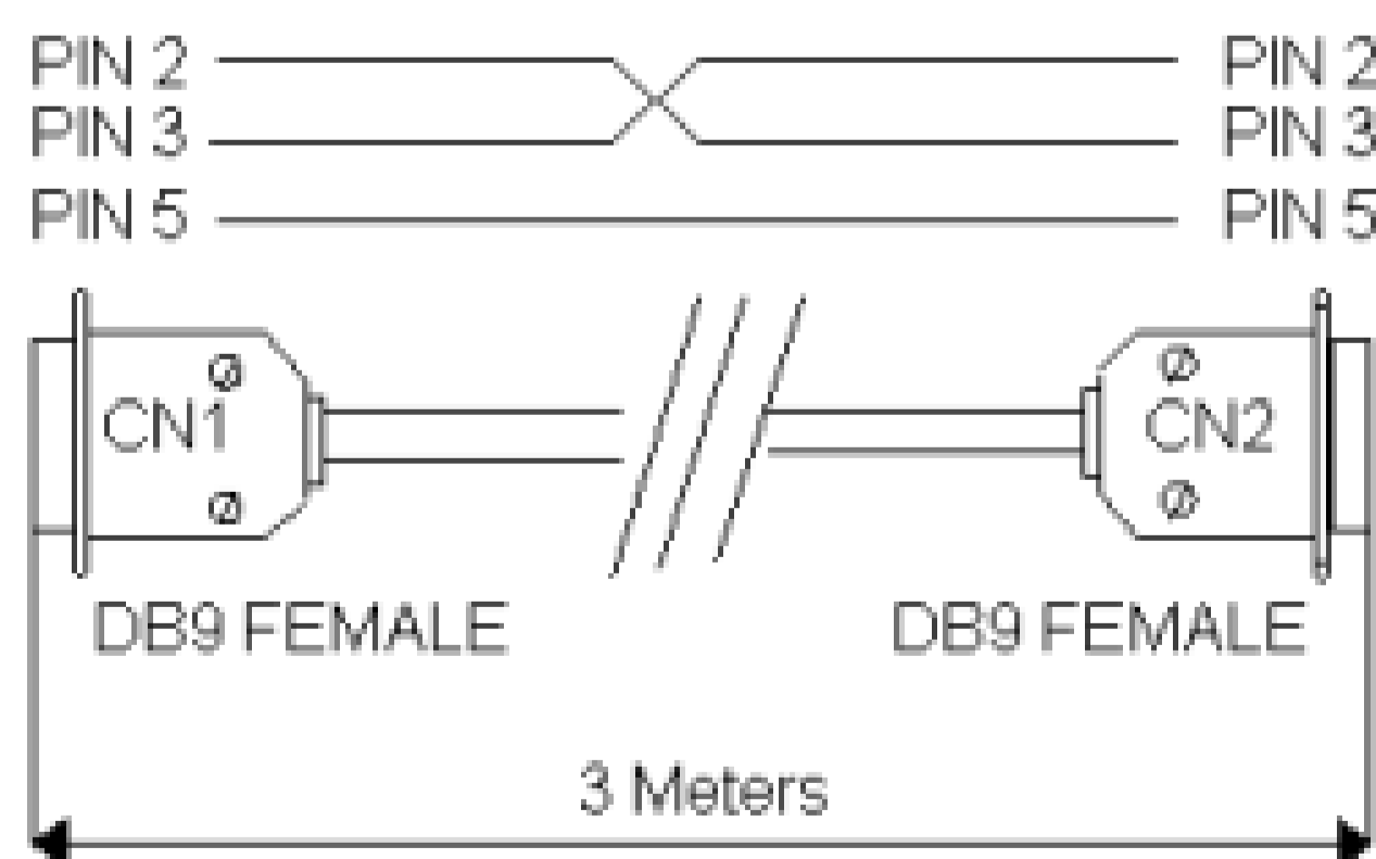
Figure 15 PC connection cable
