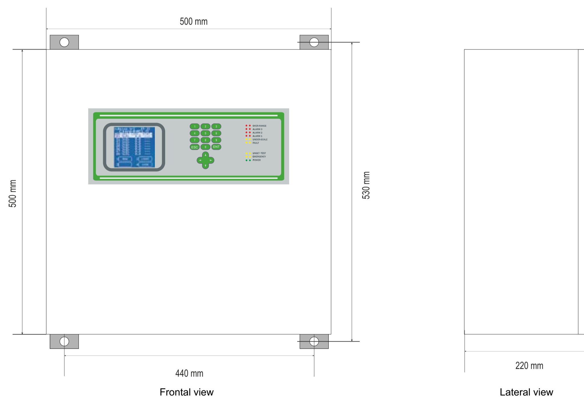
Figure 4 Dimensions of the control panel box (mm)
