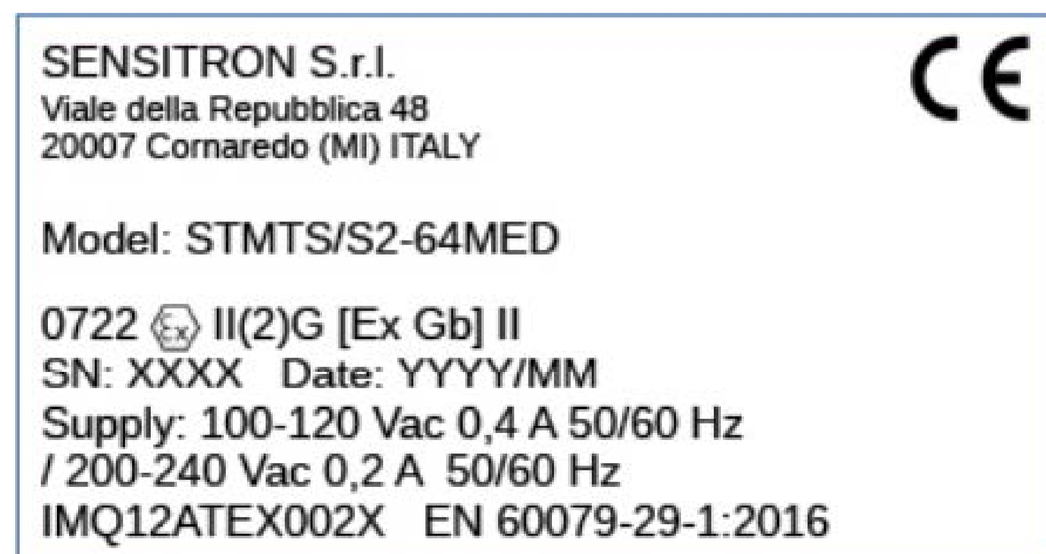
Figure 2 Example of ATEX marking, rack version
