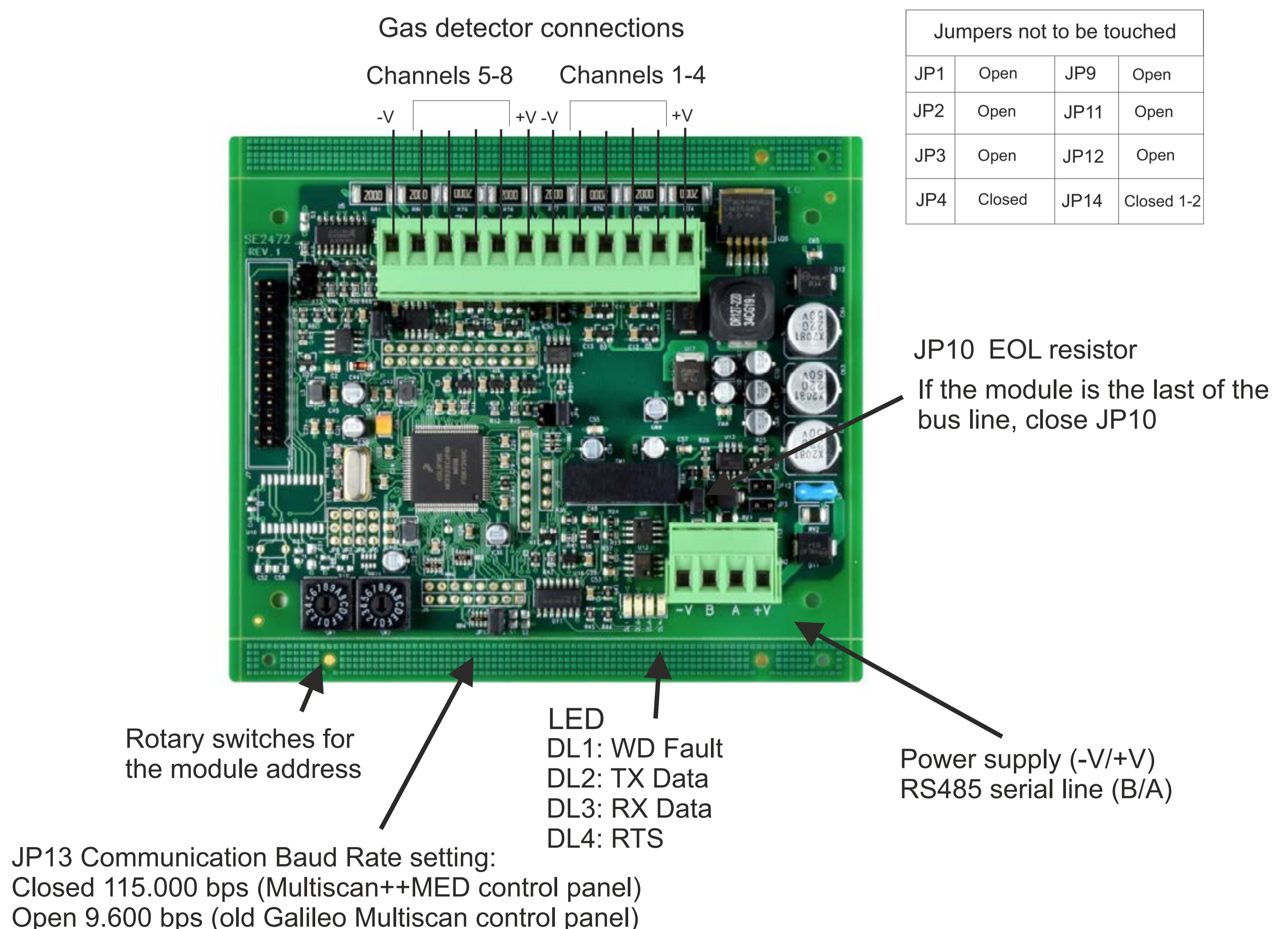
Figure 10 STG/IN8-S2MED module
