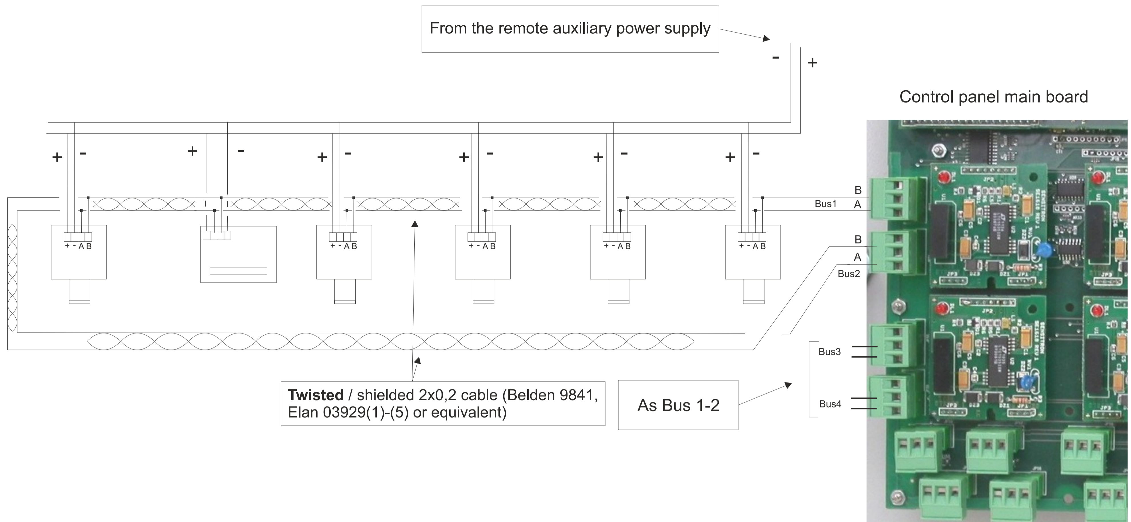
Figure 9 RS485 bus devices connection
