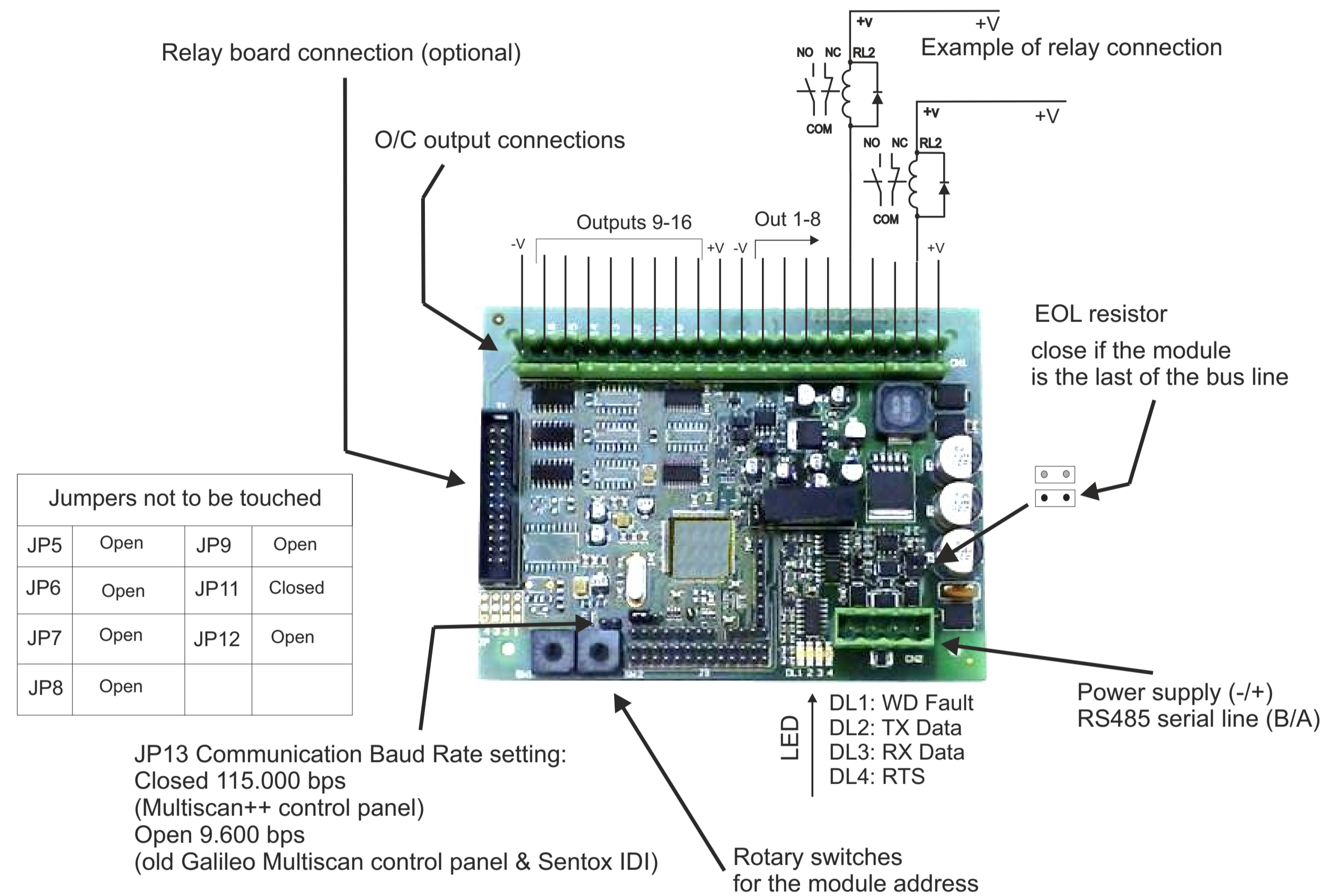
Figure 11 STG/OUT16-S2MED module
