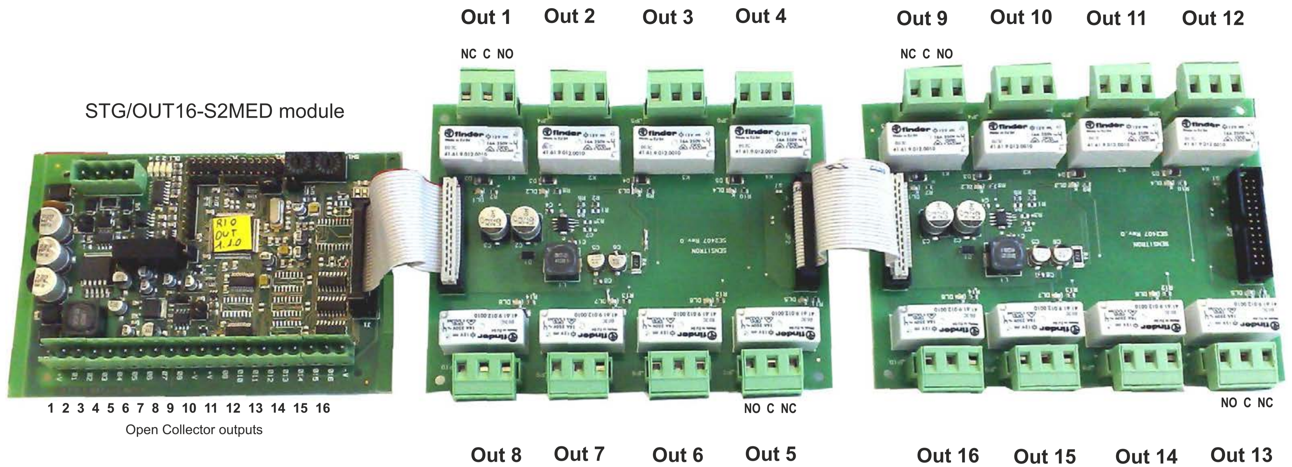
Figure 12 Relay board connection to the output module
