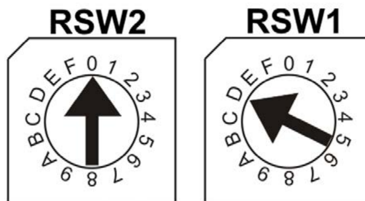
Figure 13 Example: If the address switches are set in this manner, RSW2 at 0 and RSW1 at D, the corresponding address in decimal number would be 13 (see table below).
