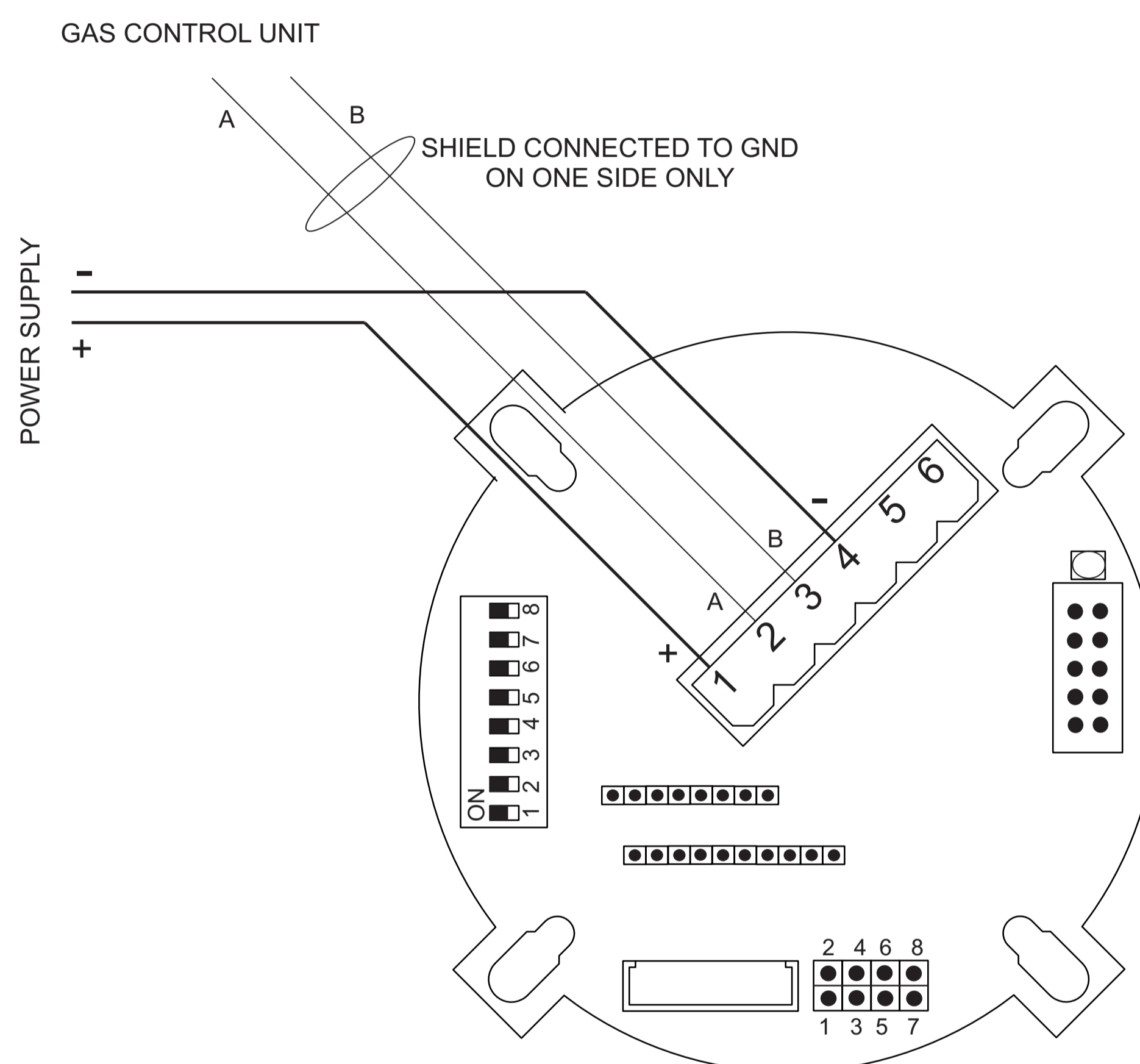
Figure 3: Detector connection to RS485 bus lines
